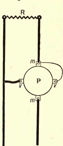
Fig. 213.—Connections of Phasemeter to Two-Wire Circuit
